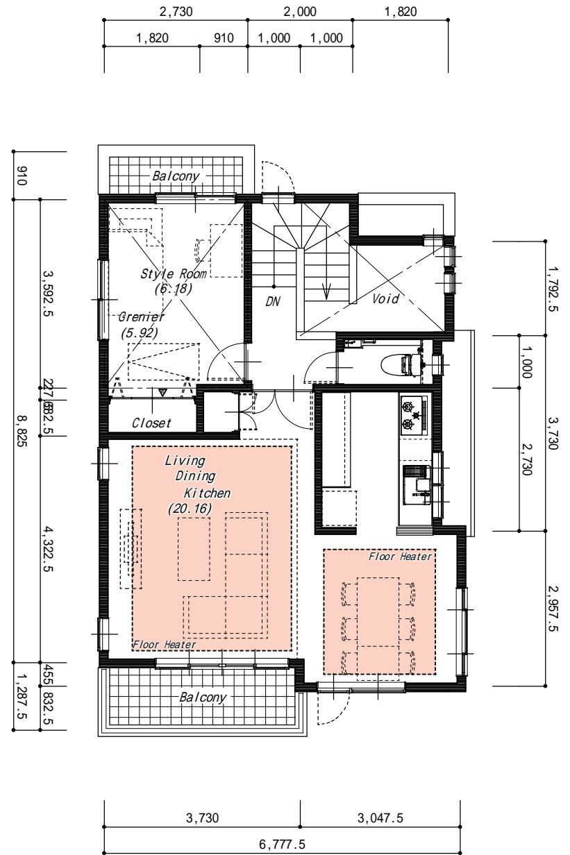
2 F PLAN
