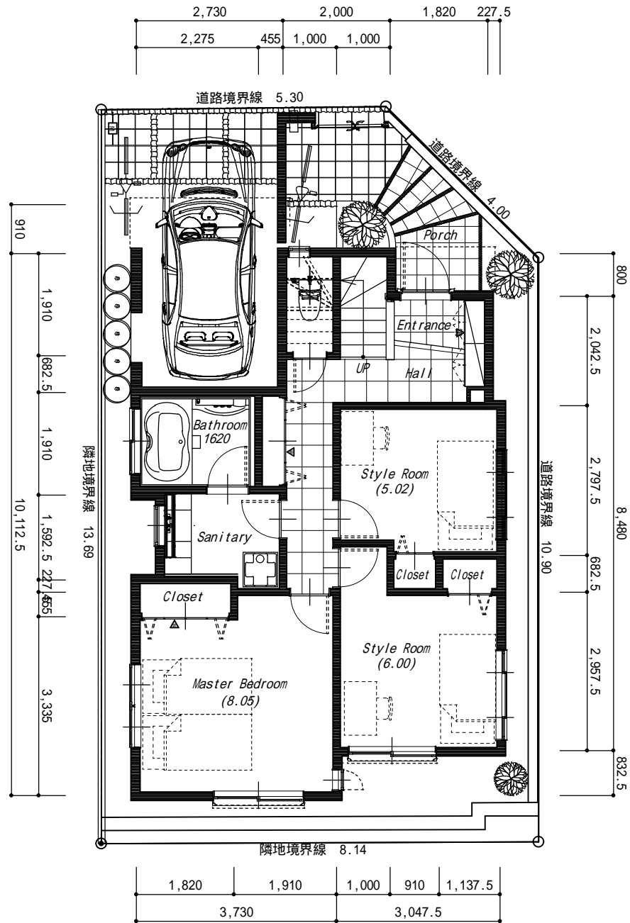
1 F PLAN
