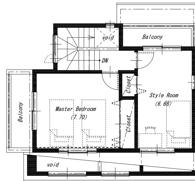
3F PLAN
