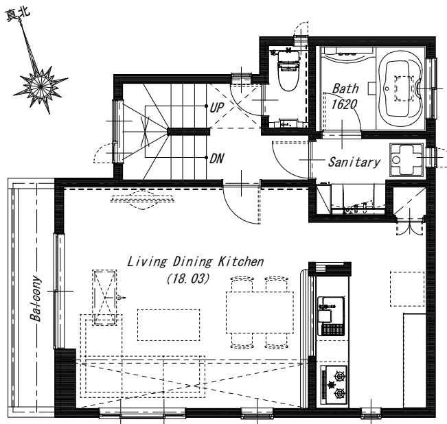
2F PLAN
