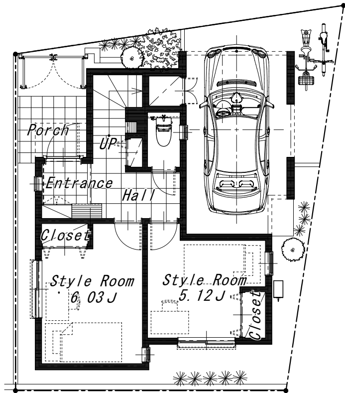
1 F PLAN
